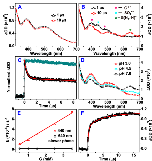
Figure 1. Transient UV-vis spectra for buffer solution (pH = 7.0) of (A) dG (3 mM) + Na_2S_2O_8 (120 mM). (B) G-quadruplex AG_3(T_2AG_3)_3 ( [G] = 1.5 mM) + Na_2S_2O_8 (120 mM) upon 355 nm laser flash photolysis. (C) Kinetics trace at 440 nm after excitation of Na_2S_2O_8 (120 mM) solution in the absence (green circle) or presence (black circle) of G-quadruplex AG_3(T_2AG_3)_3 ( [G] = 1.5 mM), with the single-exponential fit to the data (red solid line). (D) Transient UV-vis spectra at 10 \mu s after excitation of (B) solution at pH 3.0 (red circle), 4.5 (blue triangle), and 7.0 (black square). (E) Concentration dependence for the rate constants obtained from the fast decay of 440 nm band (red triangle) and the slower phase increase of 640 nm band (black circle), respectively. (F) Kinetics trace at 640 nm after excitation of (B) solution, with the double-exponential fits to the data (solid line).
